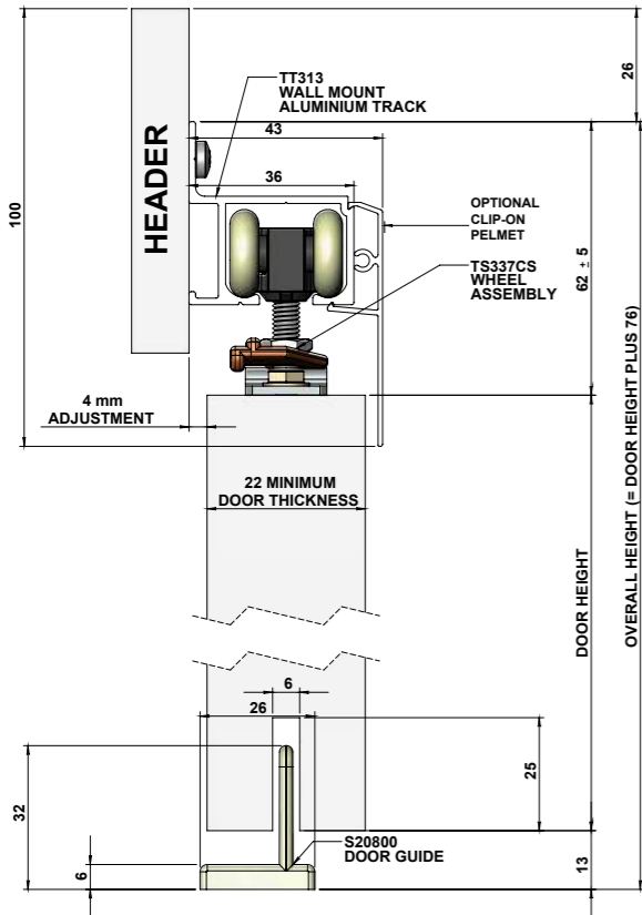
END VIEW - WALL MOUNT
