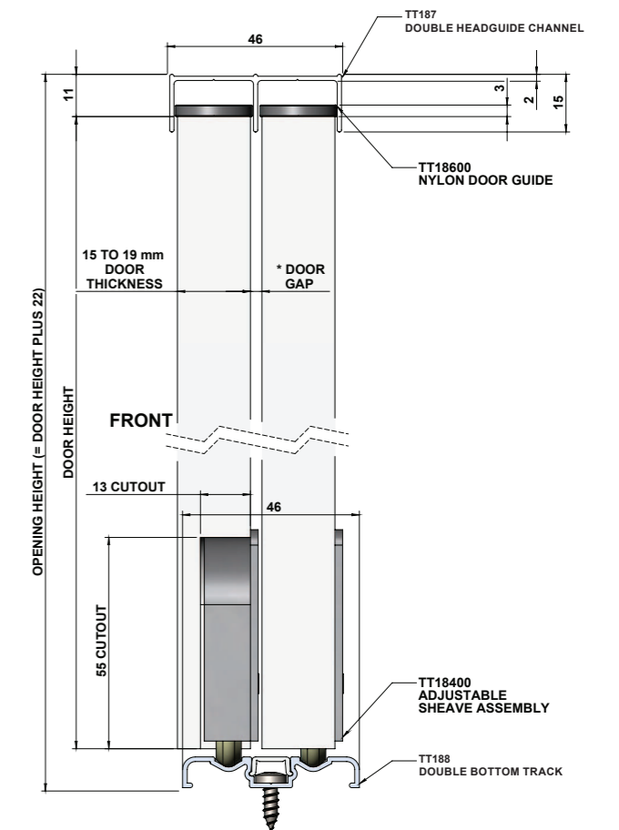
END VIEW
