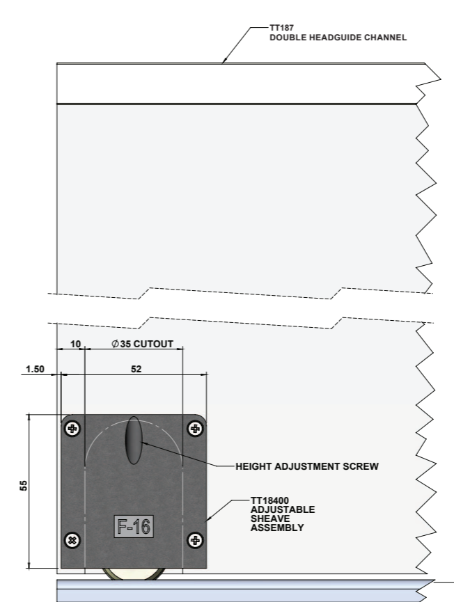
BACK VIEW
